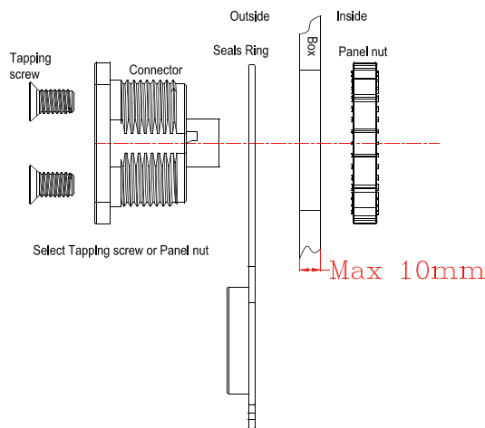
Installation method
